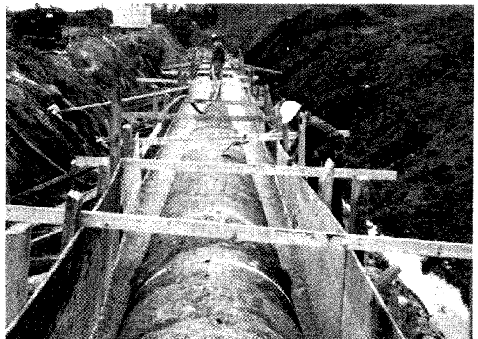
Ultra-Lite 280 pumped 3700 feet from one location as a pipe bedding in unstable soil.
