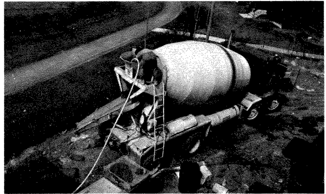
Terra-Fill contractor surcharging a transit. Truck grout mix with Cellofoam*.
